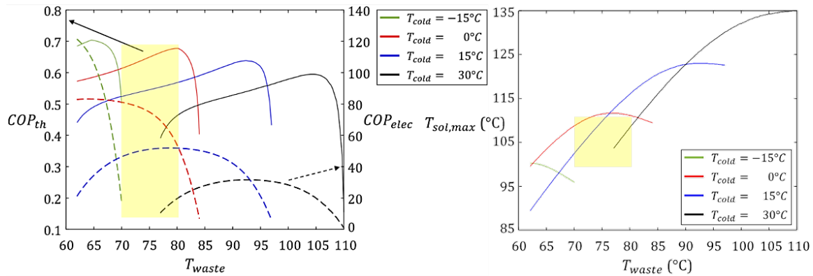
Figure 5: Operating range of an ammonia-water AHT. Estimated performance (left) and maximum solution temperature reached inside the absorber until it reaches saturation (right) as a function of the cold heat rejection ( T_{cold} ) and the waste heat ( T_{waste} ) temperatures (Source: Collignon et al., 2025). The yellow-highlighted regions indicate the operating range of the ZIMBA AHT.
