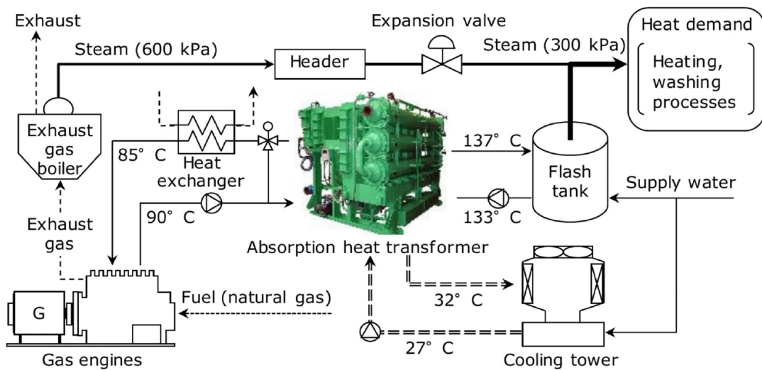
Figure 9: AHT installed in an industrial plant (capacity: 150 kW) (Cudok et al., 2021; Fujii et al., 2008).
